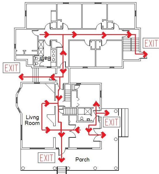
1st Floor Evacuation Map
